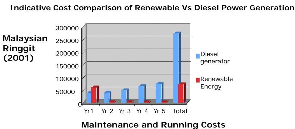
Fig. 4: Indicative Cost Comparison of Renewable versus Diesel Power Generation
