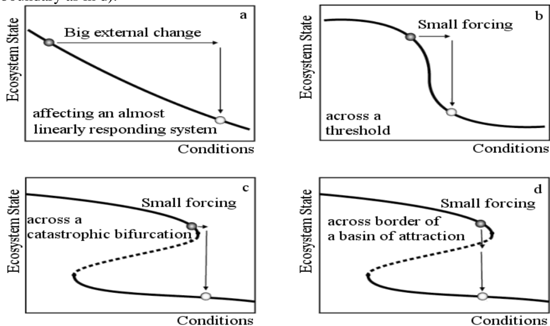
Figure:5 The state of a system responds to a change in conditions. The continuous line represents a stable equilibria. In a) a change in conditions drives an approximately linear response in the systems state, unlike b) where a threshold is crossed and the relationship becomes very sensitive. The fold bifurcation (c,d) has three equilibria for the same condition, but one represented by the dotted line is unstable. That means that there is a range of system states which are dynamically unstable to any condition 53 .
